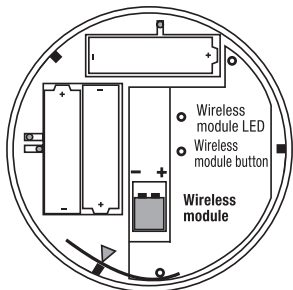
Polarity of batteries and control elements on the rear of the device
